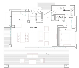
IDIRO 4 - BAR GROUND FLOOR
