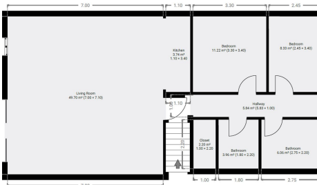
nd Floor TOTAL AREA: 91.01 m 2
