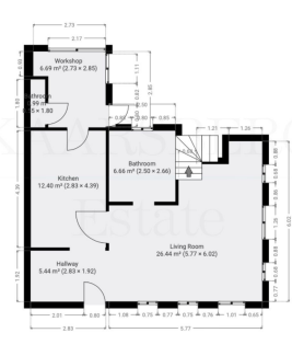
10 FT TO SCALE West house - 1st floor
