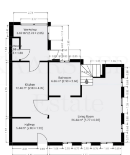
10 FT TO SCALE West house - 1st floor
